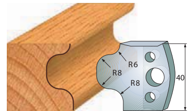
Pair of knives 690.056 Pair of limiters 691.056
