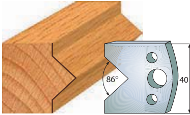
Pair of knives 690.034 Pair of limiters 691.034
