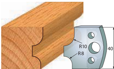
Pair of knives 690.040 Pair of limiters 691.040
