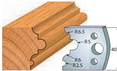
Pair of knives 690.036 Pair of limiters 691.036
