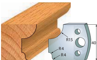
Pair of knives 690.043 Pair of limiters 691.043
