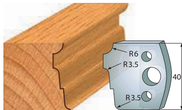
Pair of knives 690.039 Pair of limiters 691.039
