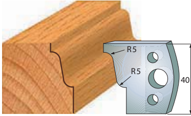
Pair of knives 690.031 Pair of limiters 691.031
