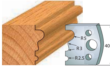
Pair of knives 690.033 Pair of limiters 691.033
