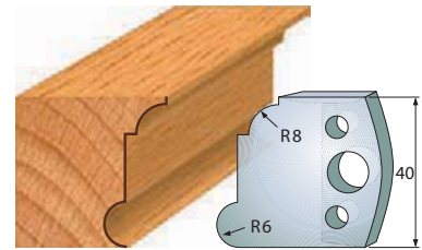
Pair of knives 690.053 Pair of limiters 691.053
