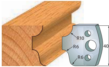
Pair of knives 690.045 Pair of limiters 691.045
