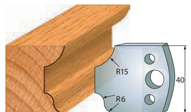
Pair of knives 690.044 Pair of limiters 691.044
