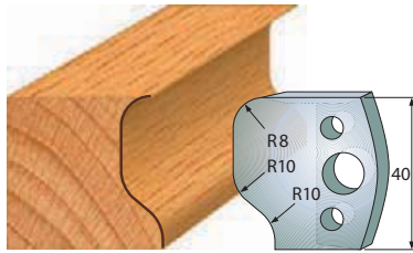
Pair of knives 690.049 Pair of limiters 691.049
