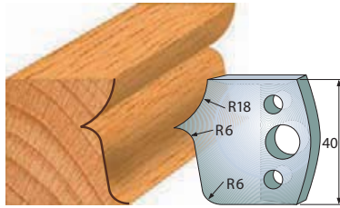
Pair of knives 690.046 Pair of limiters 691.046
