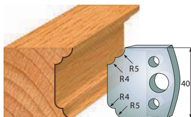
Pair of knives 690.042 Pair of limiters 691.042
