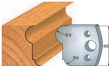
Pair of knives 690.055 Pair of limiters 691.055
