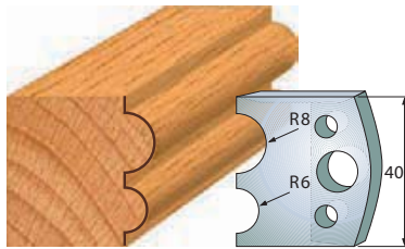
Pair of knives 690.051 Pair of limiters 691.051
