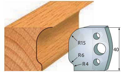
Pair of knives 690.047 Pair of limiters 691.047
