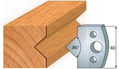
Pair of knives 690.035 Pair of limiters 691.035
