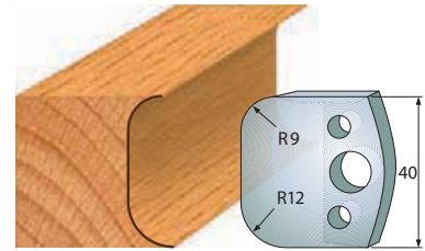
Pair of knives 690.050 Pair of limiters 691.050
