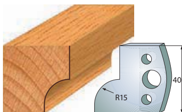
Pair of knives 690.057 Pair of limiters 691.057
