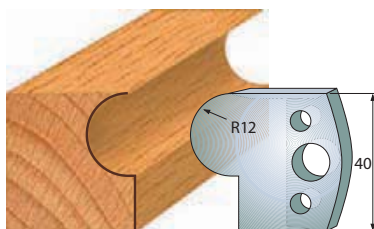
Pair of knives 690.058 Pair of limiters 691.058
