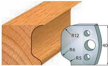
Pair of knives 690.048 Pair of limiters 691.048
