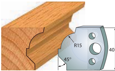
Pair of knives 690.037 Pair of limiters 691.037
