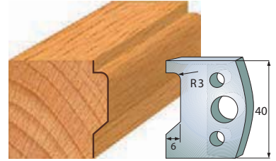
Pair of knives 690.032 Pair of limiters 691.032
