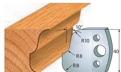
Pair of knives 690.059 Pair of limiters 691.059
