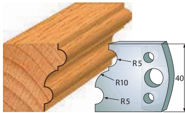
Pair of knives 690.052 Pair of limiters 691.052
